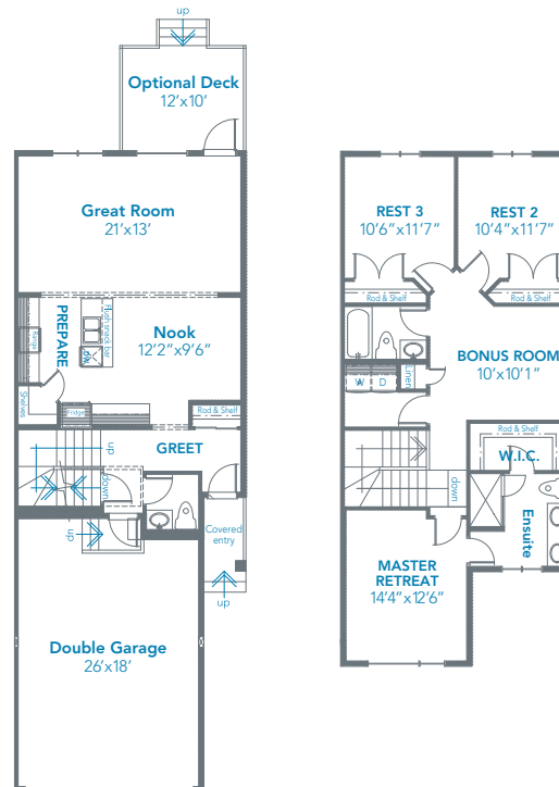
Main level 775 sq. ft.
