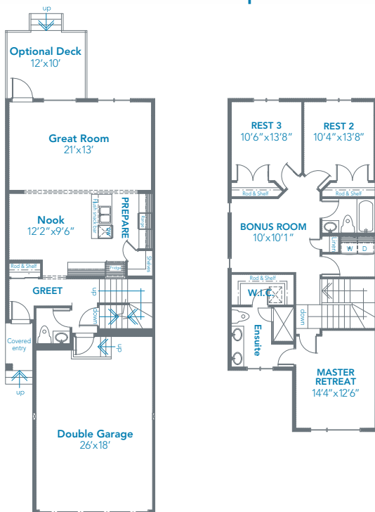
Main level 775 sq. ft.
