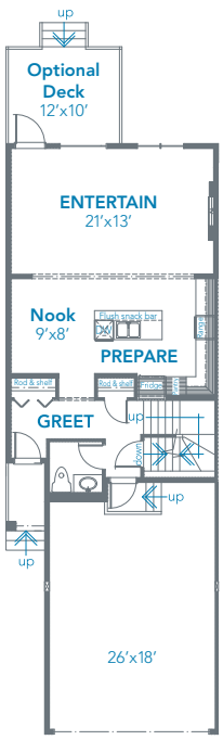
Main level 775 s.f.
